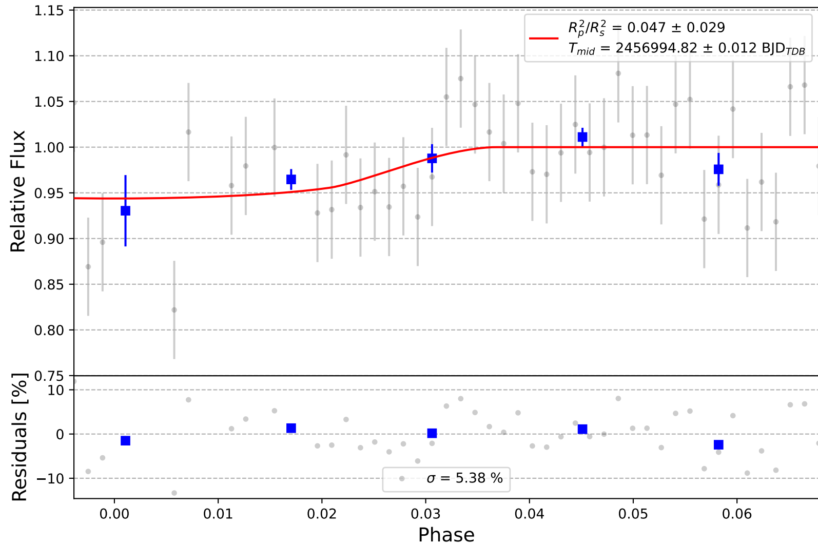
CoRoT-1 b
