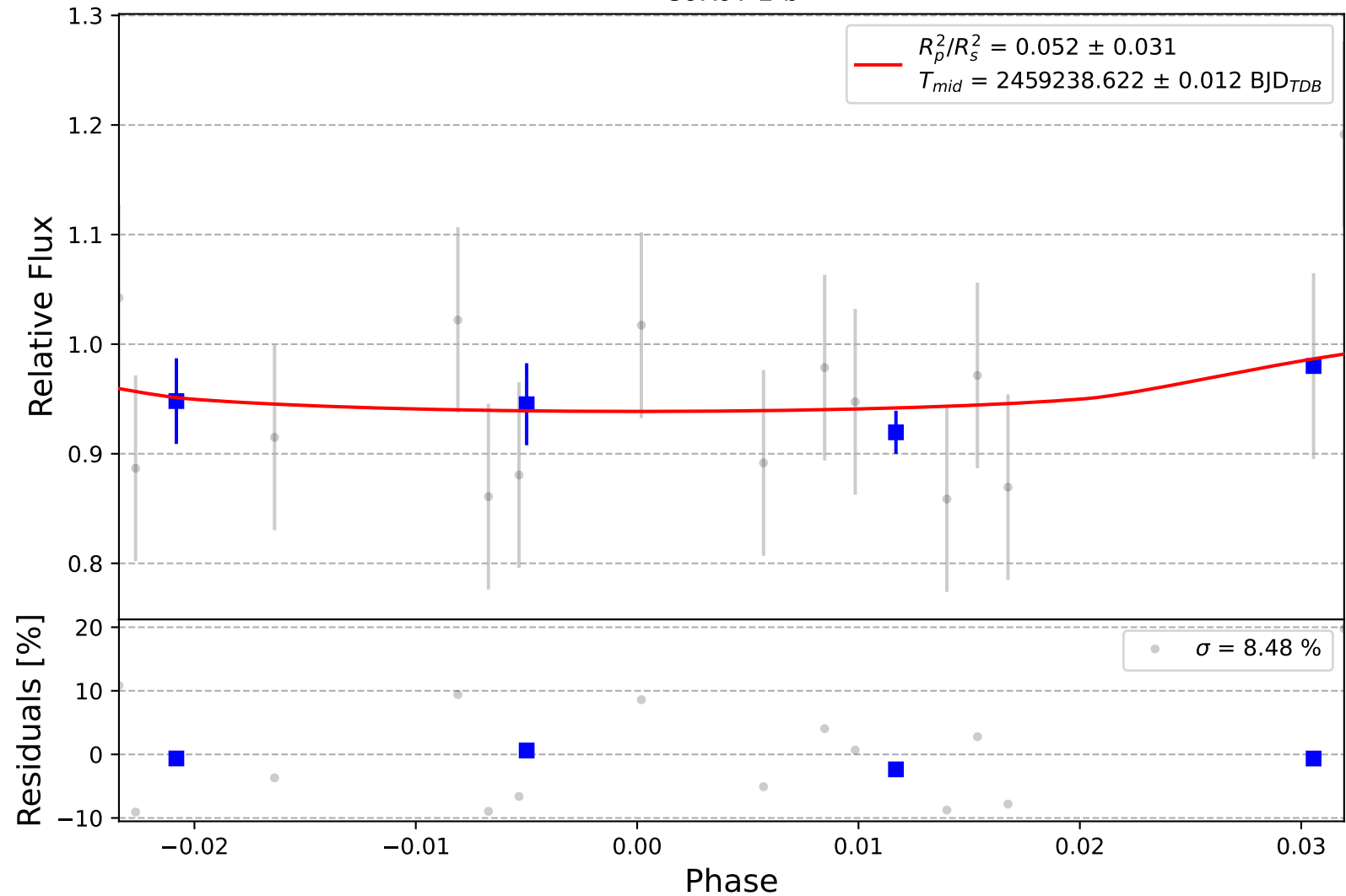
CoRoT-1 b
