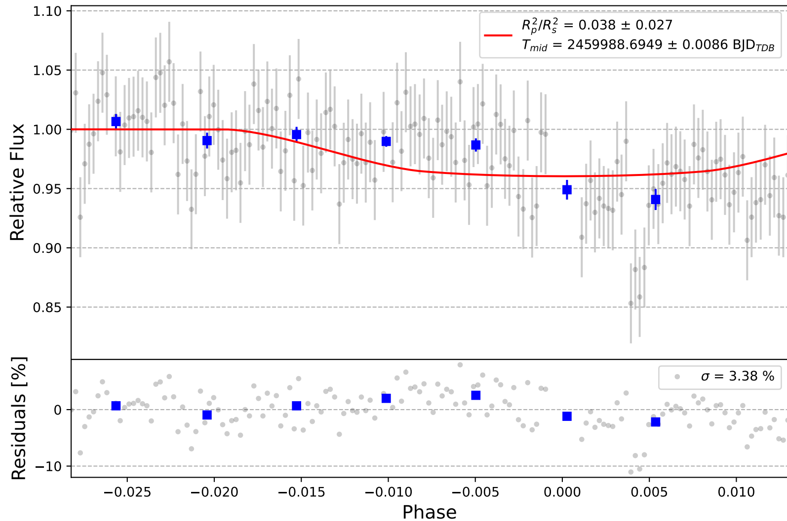
CoRoT-5 b
