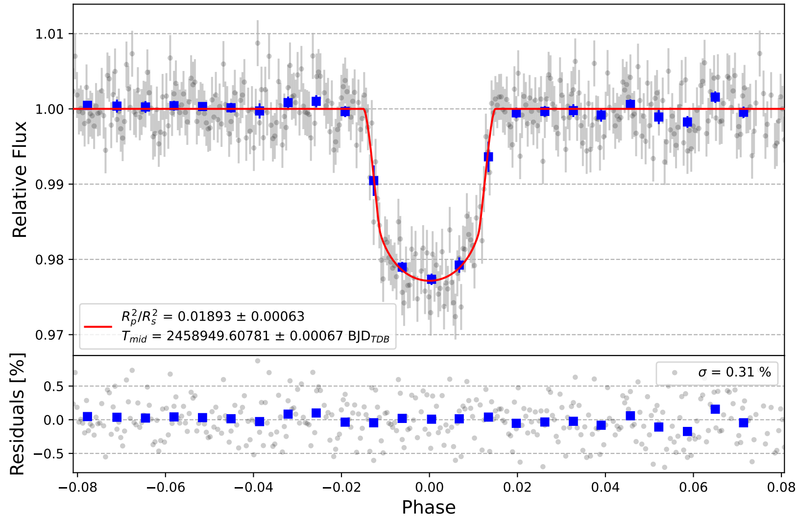
HAT-P-12 b
