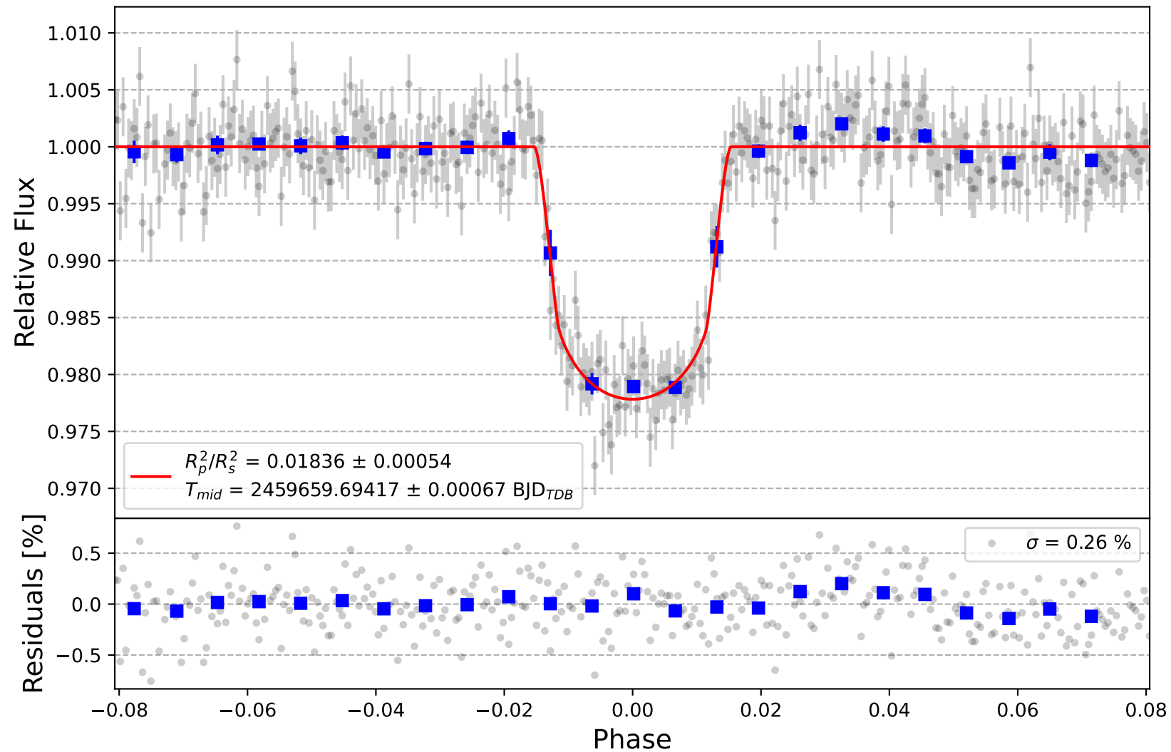
HAT-P-12 b
