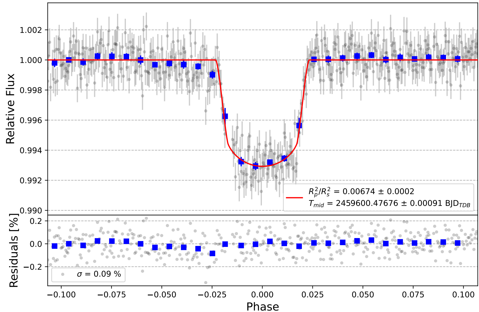
HAT-P-13 b
