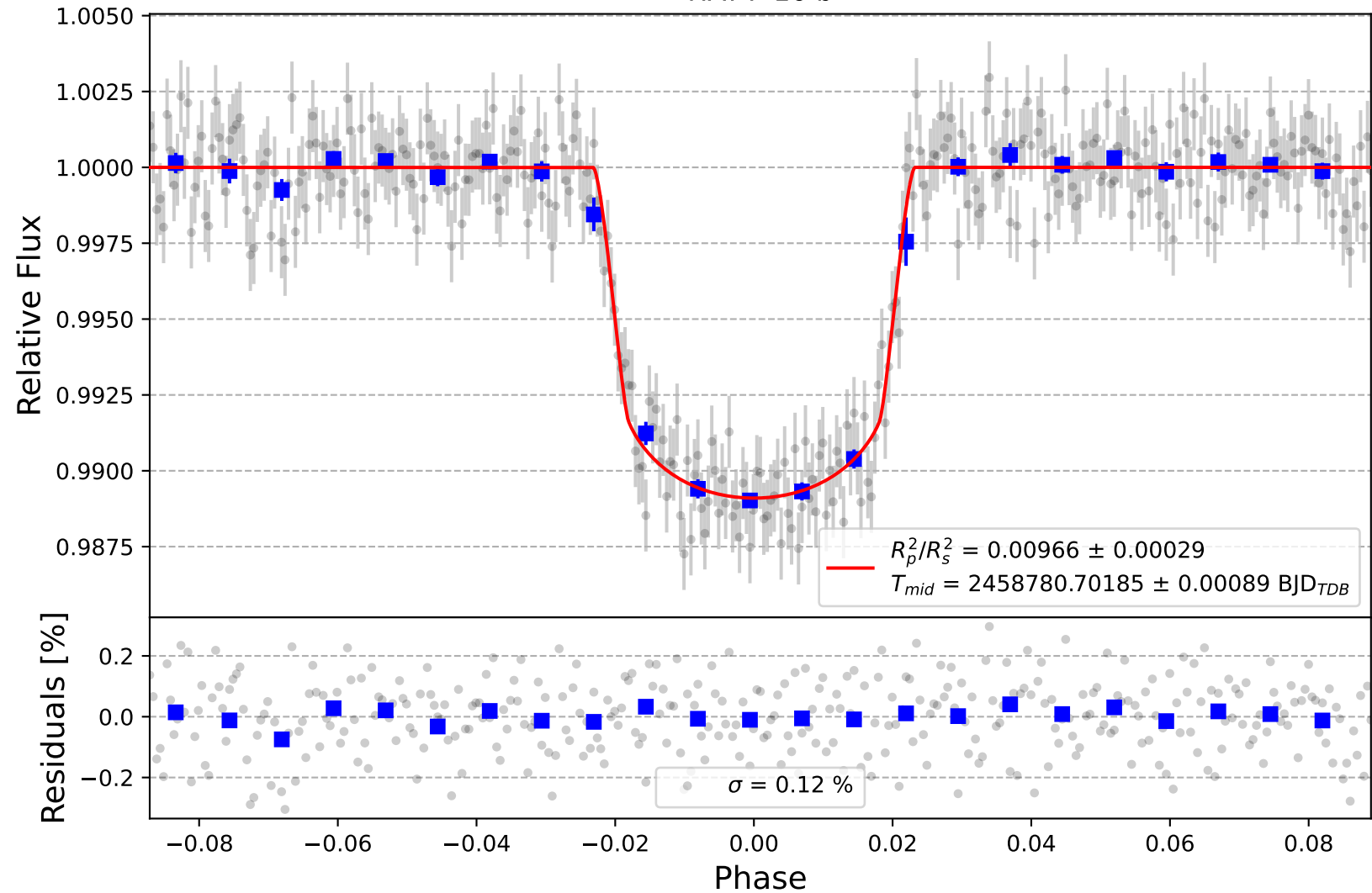
HAT-P-16 b
