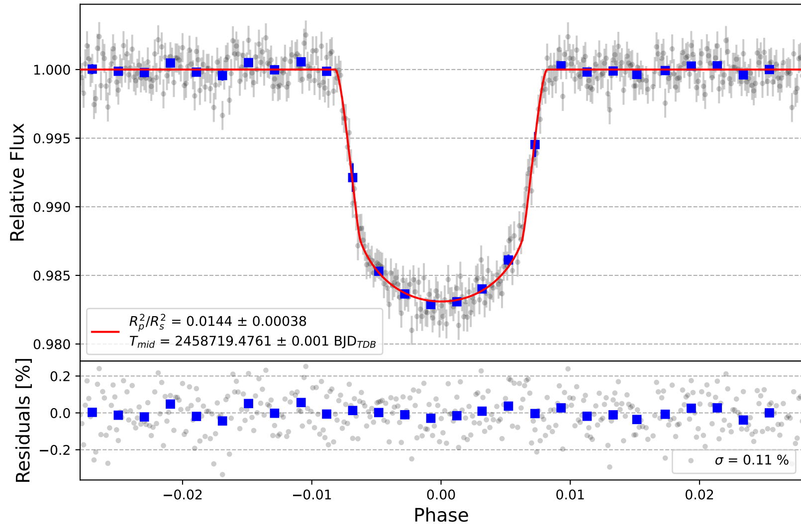
HAT-P-17 b
