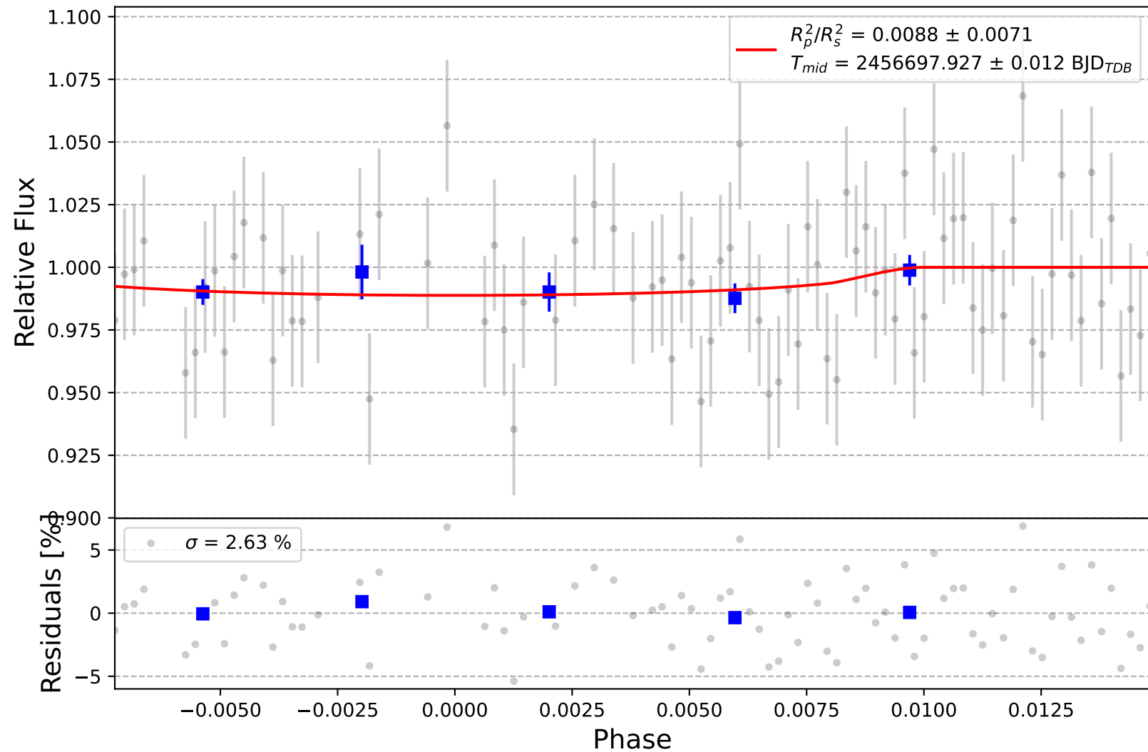
HAT-P-18 b
