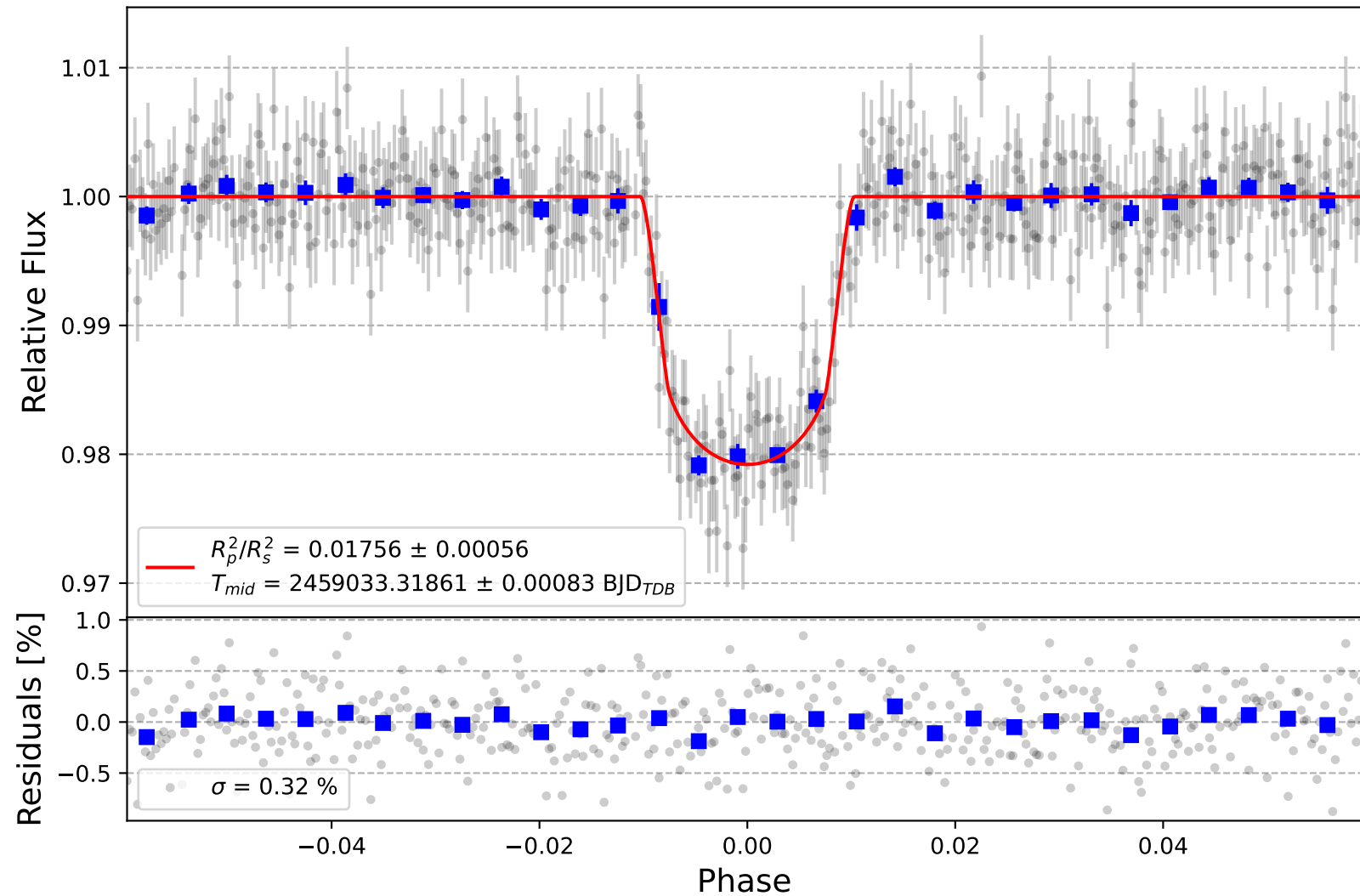
HAT-P-18 b
