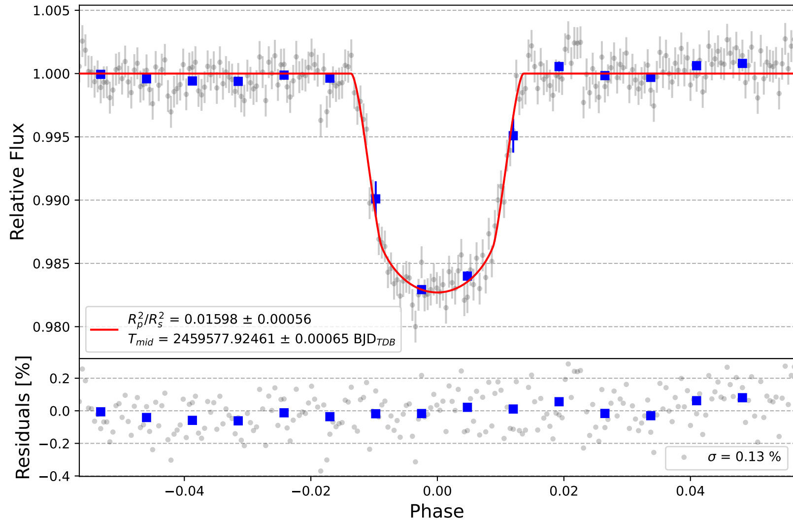
HAT-P-20 b
