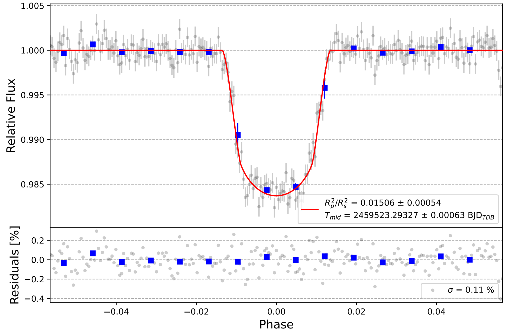
HAT-P-20 b
