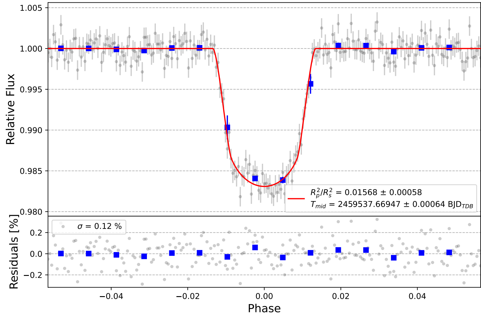
HAT-P-20 b
