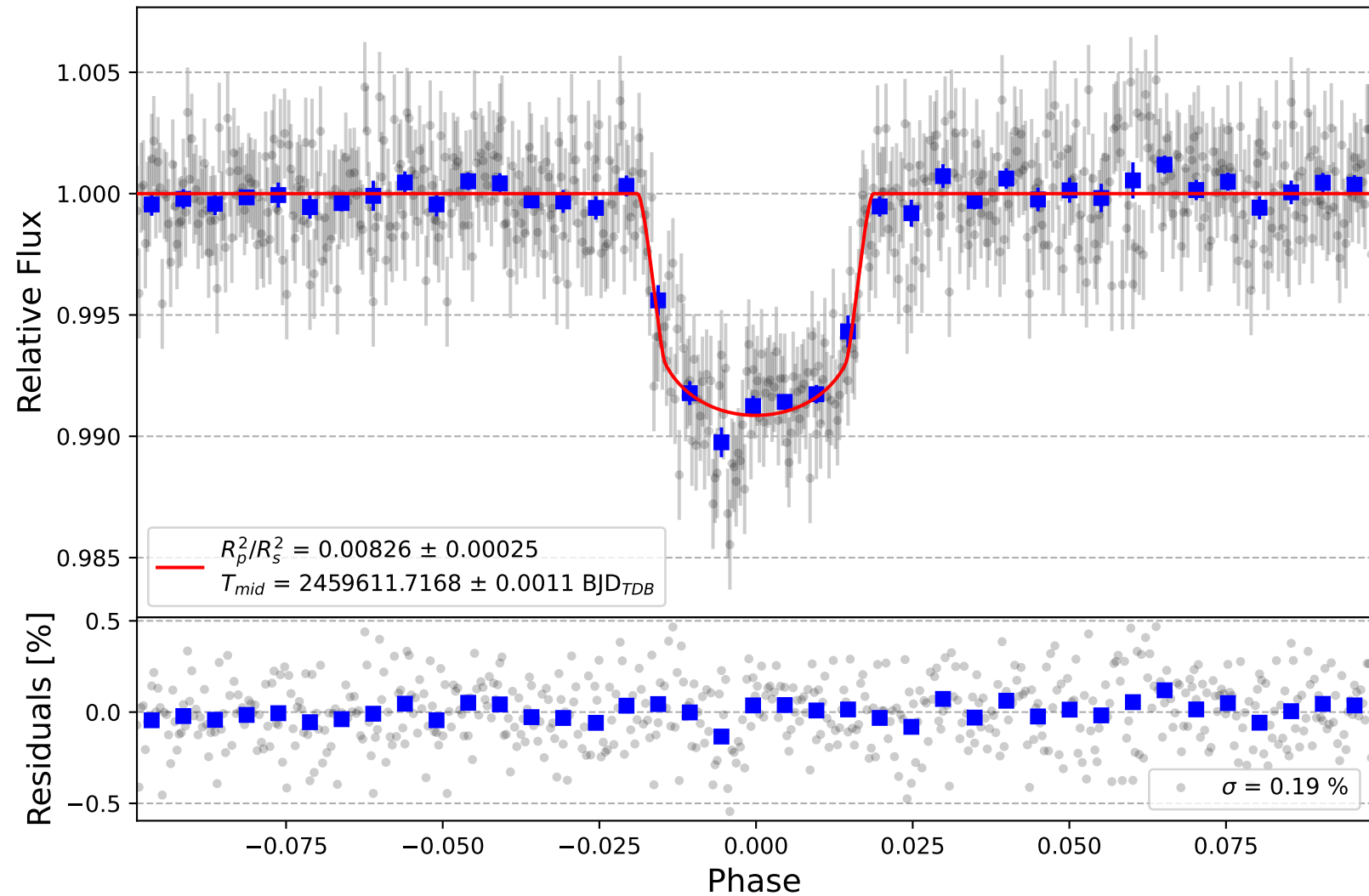
HAT-P-21 b
