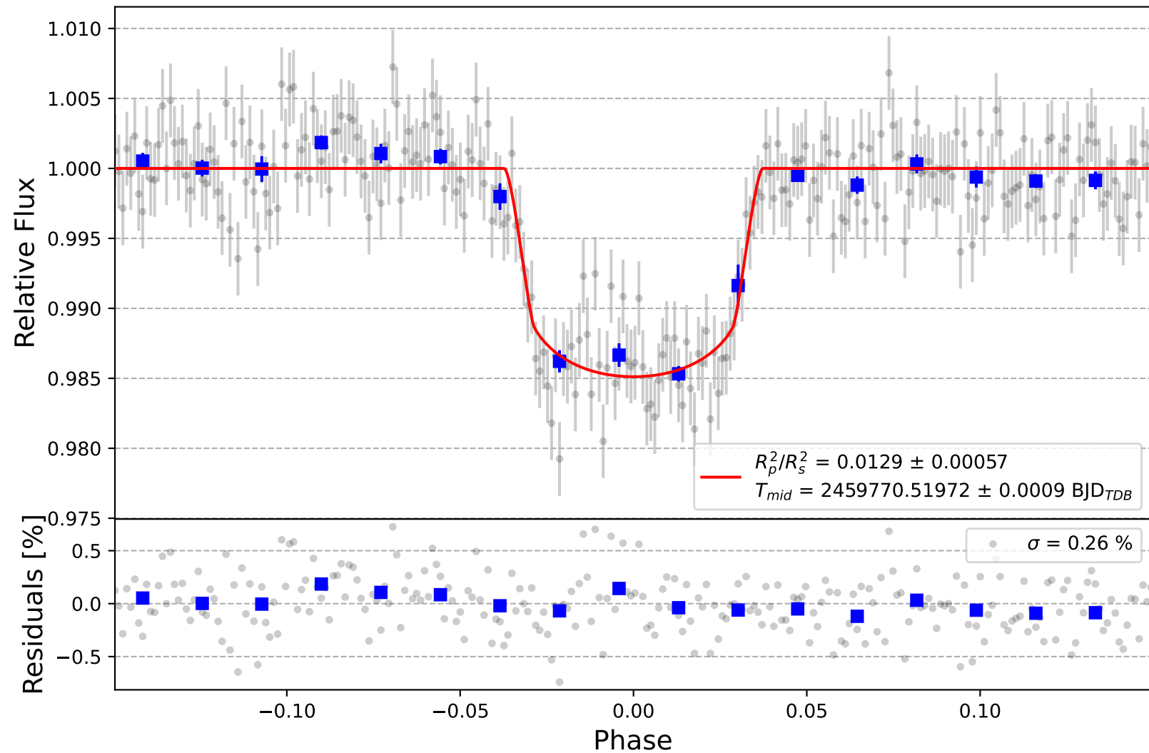
HAT-P-23 b
