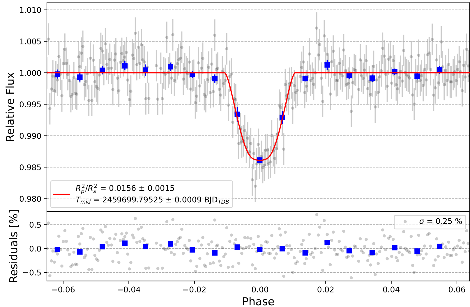
HAT-P-27 b
