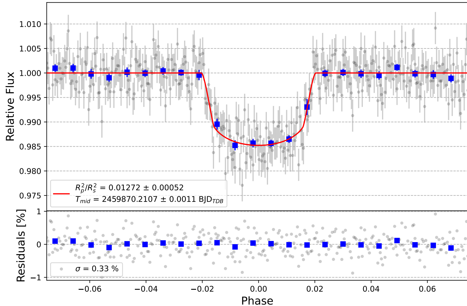
HAT-P-28 b
