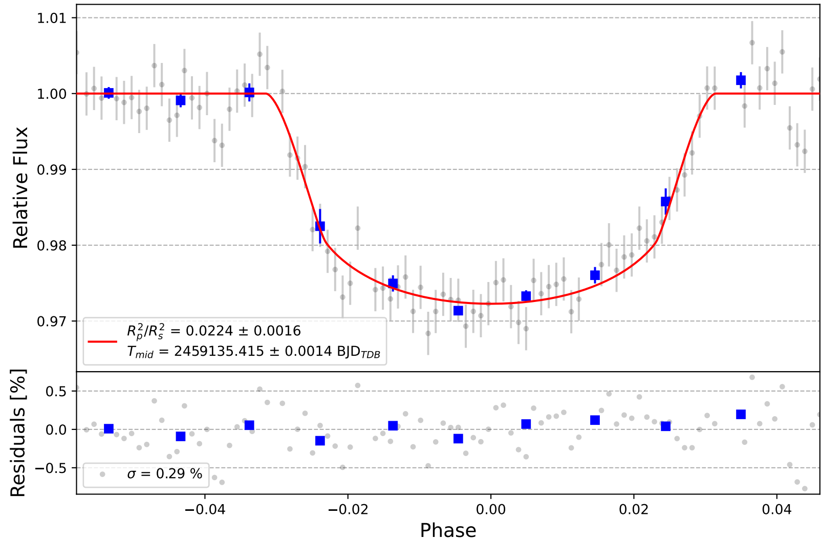
HAT-P-32 b
