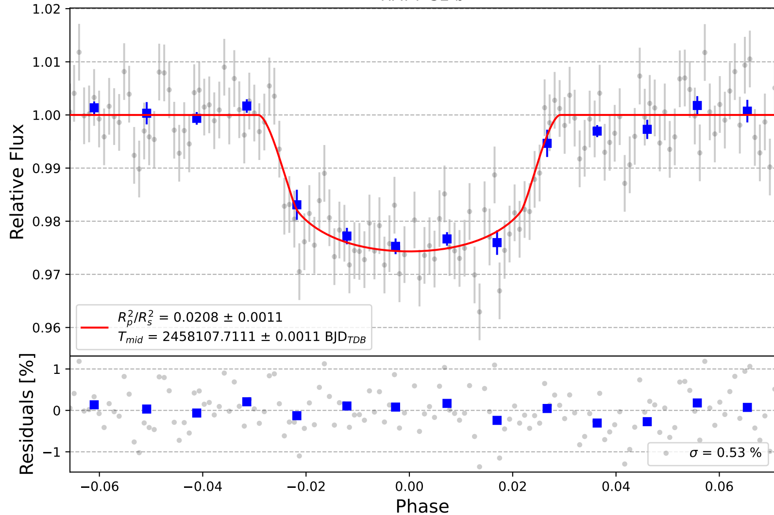
HAT-P-32 b
