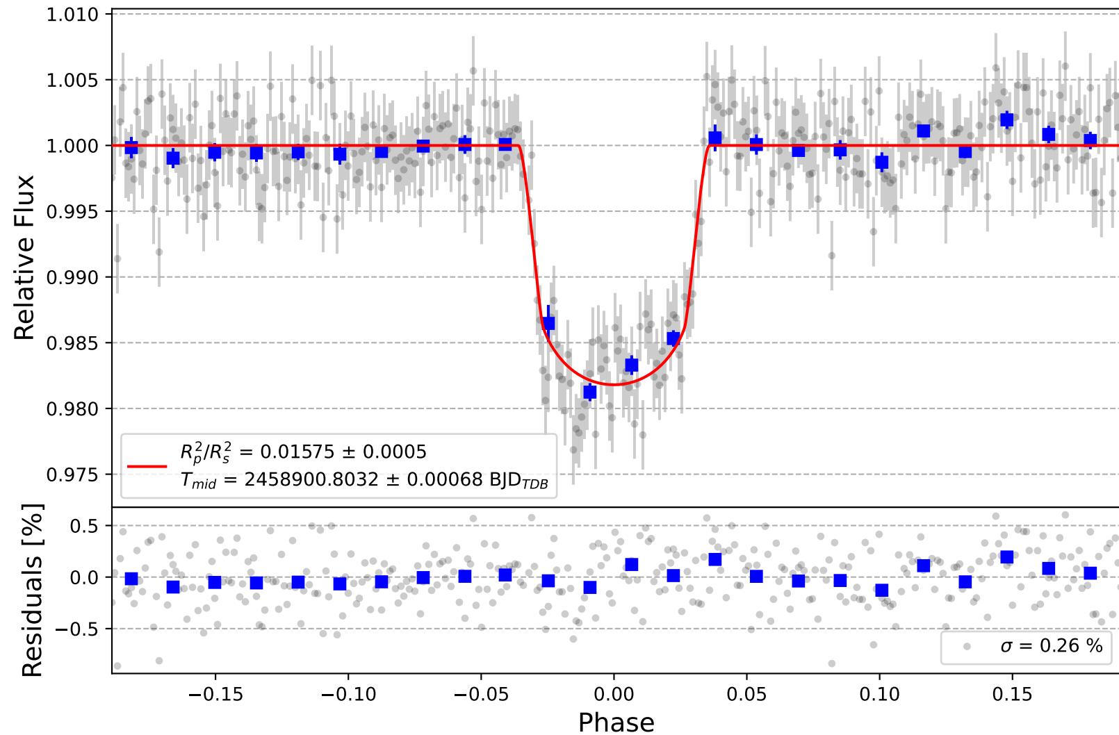
HAT-P-36 b
