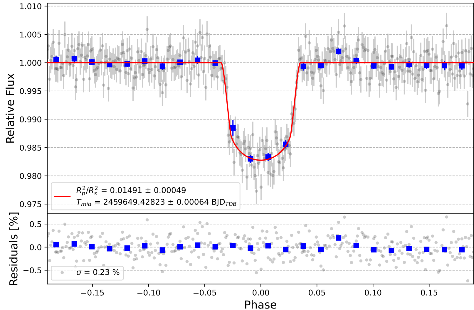
HAT-P-36 b
