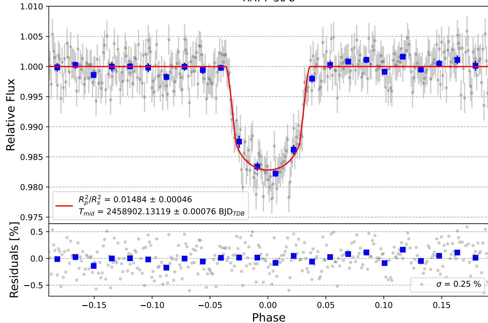
HAT-P-36 b
