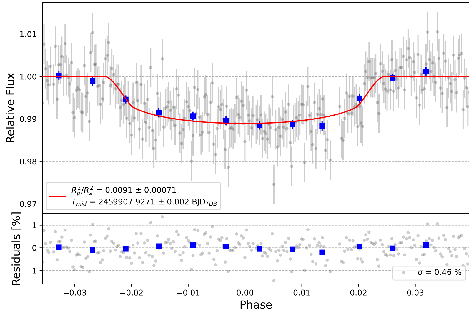
HAT-P-39 b
