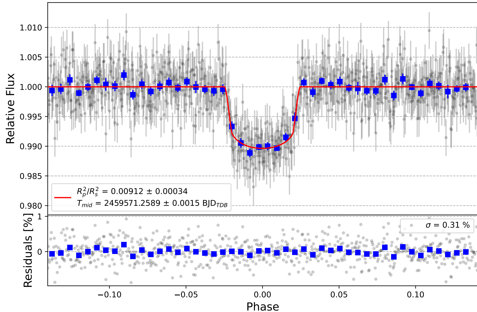
HAT-P-39 b
