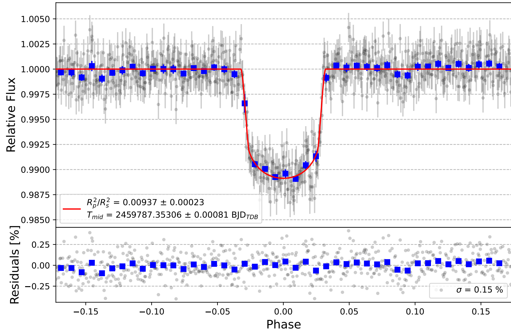
HAT-P-41 b
