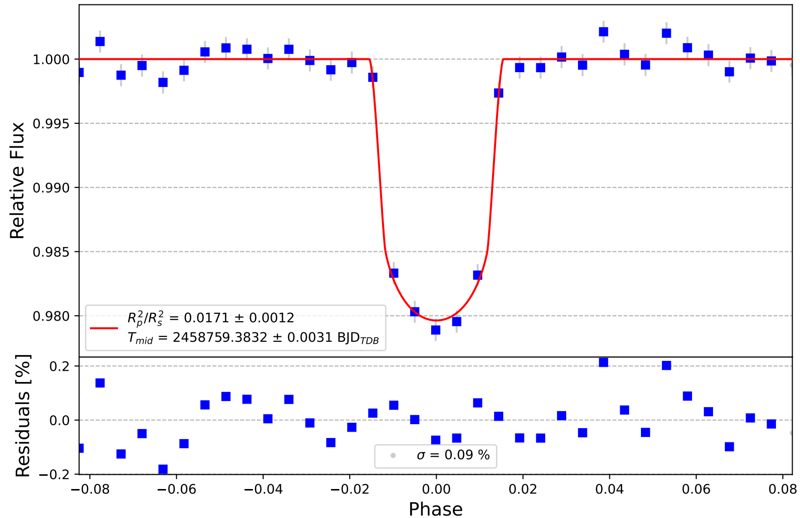
HAT-P-44 b
