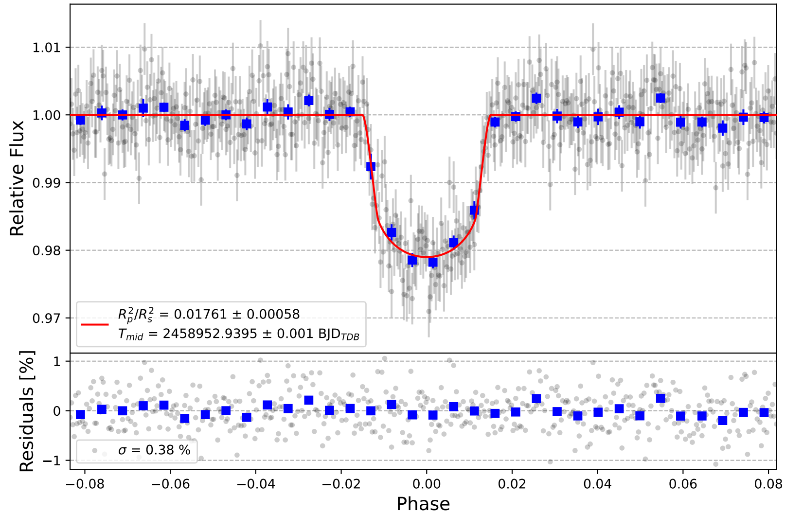
HAT-P-44 b
