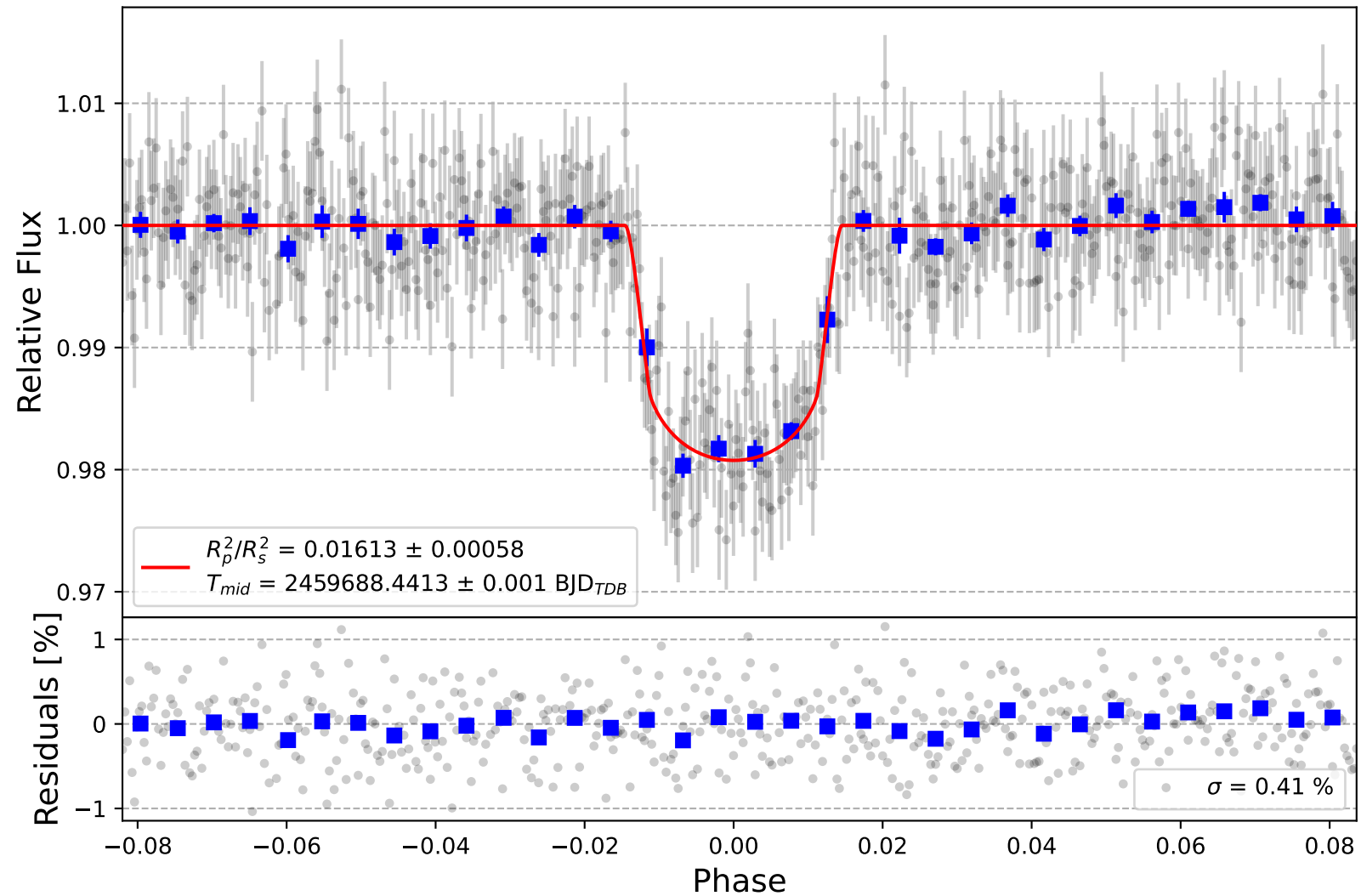
HAT-P-44 b
