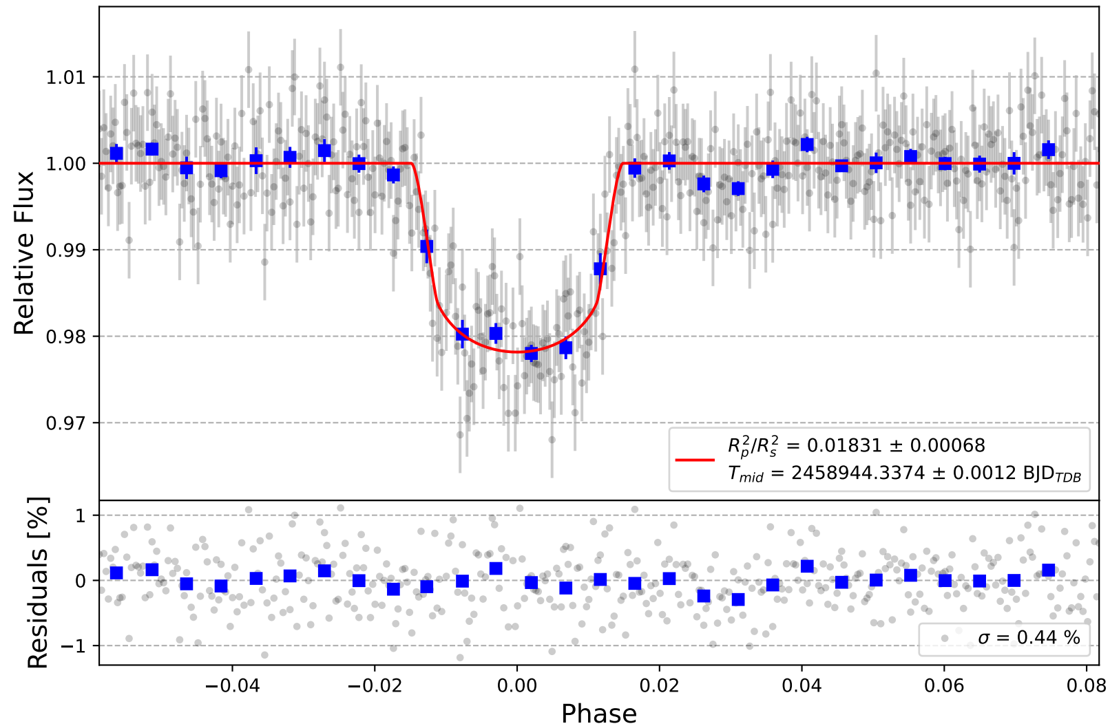
HAT-P-44 b
