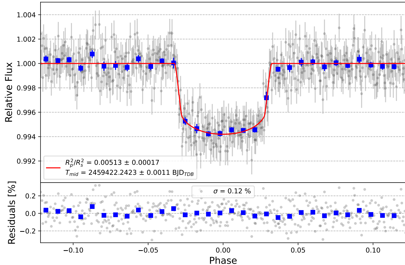
HAT-P-49 b
