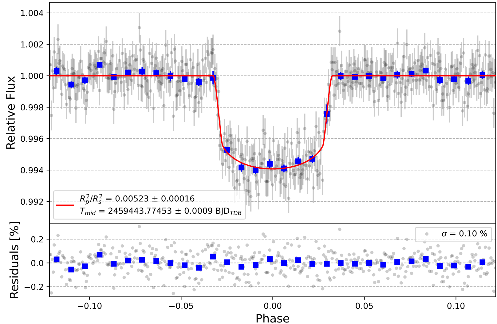
HAT-P-49 b
