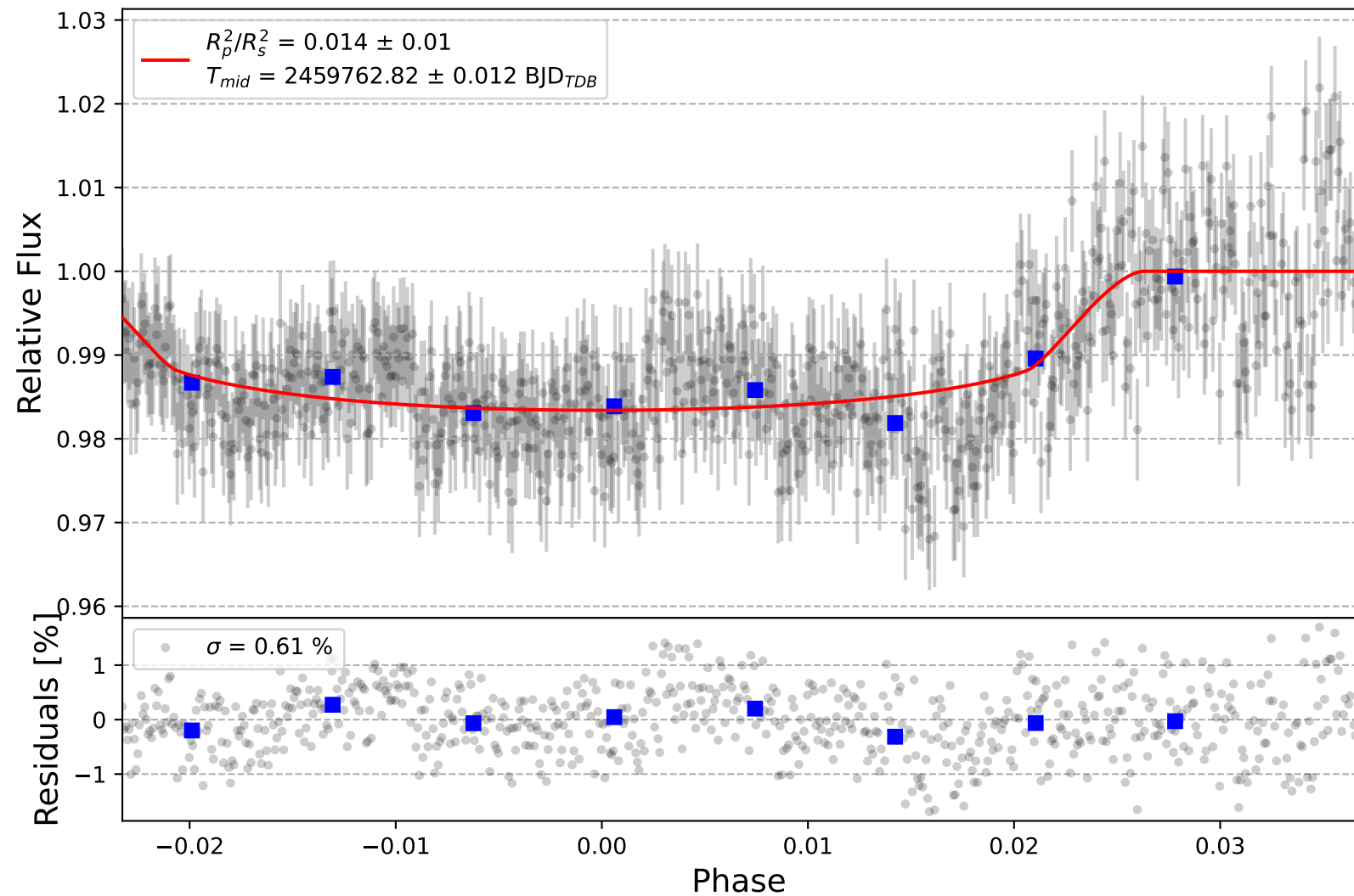
HAT-P-4 b
