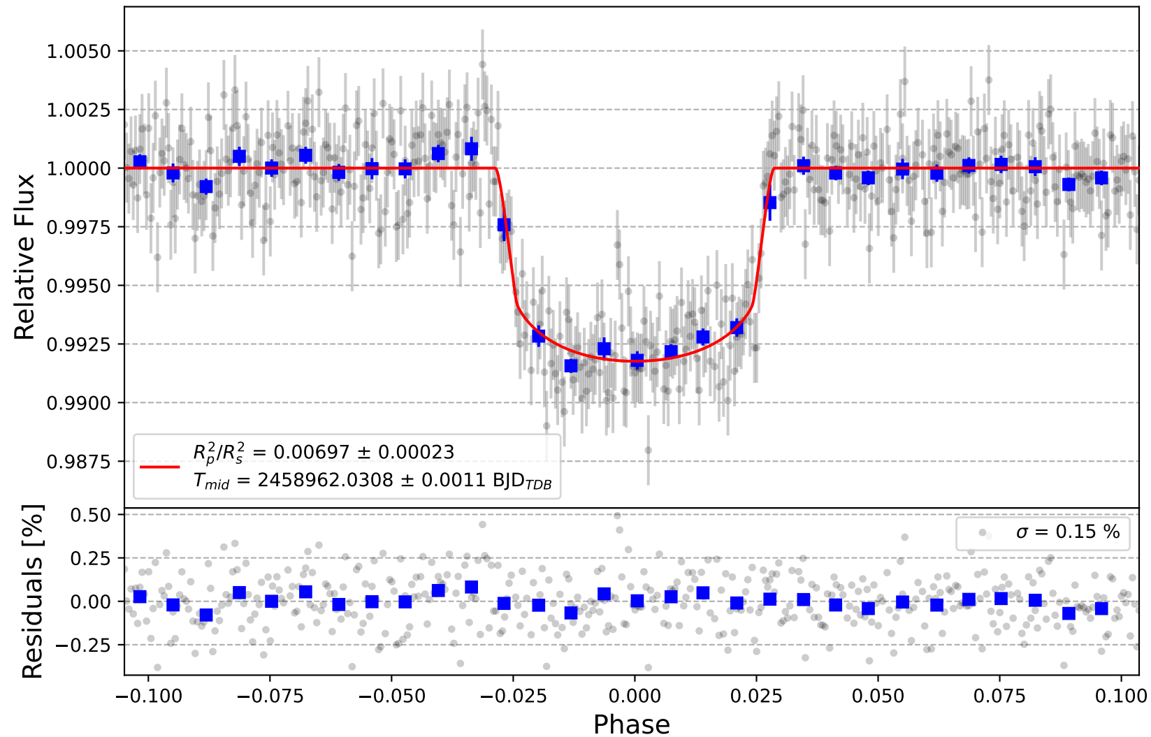
HAT-P-4 b
