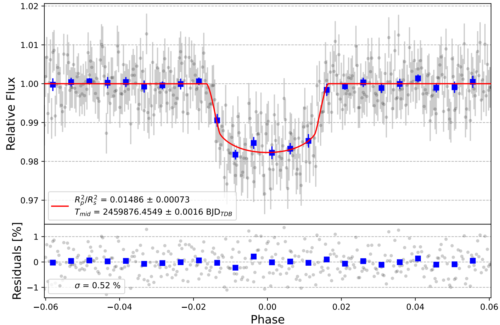
HAT-P-51 b
