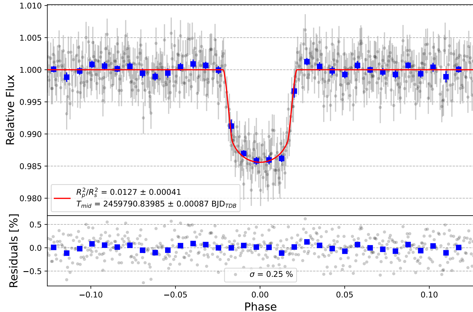
HAT-P-5 b
