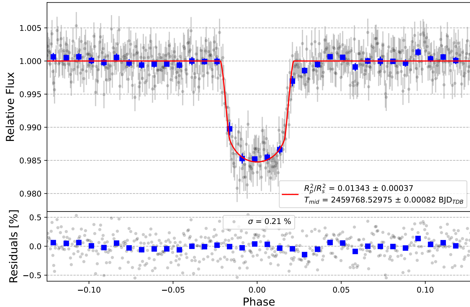
HAT-P-5 b
