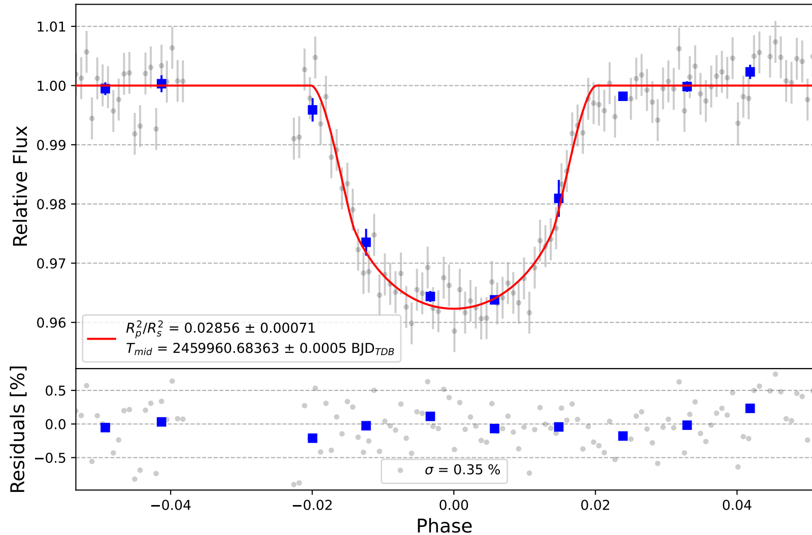
HAT-P-68 b
