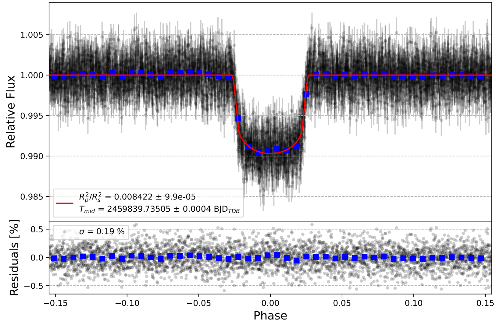
HAT-P-8 b
