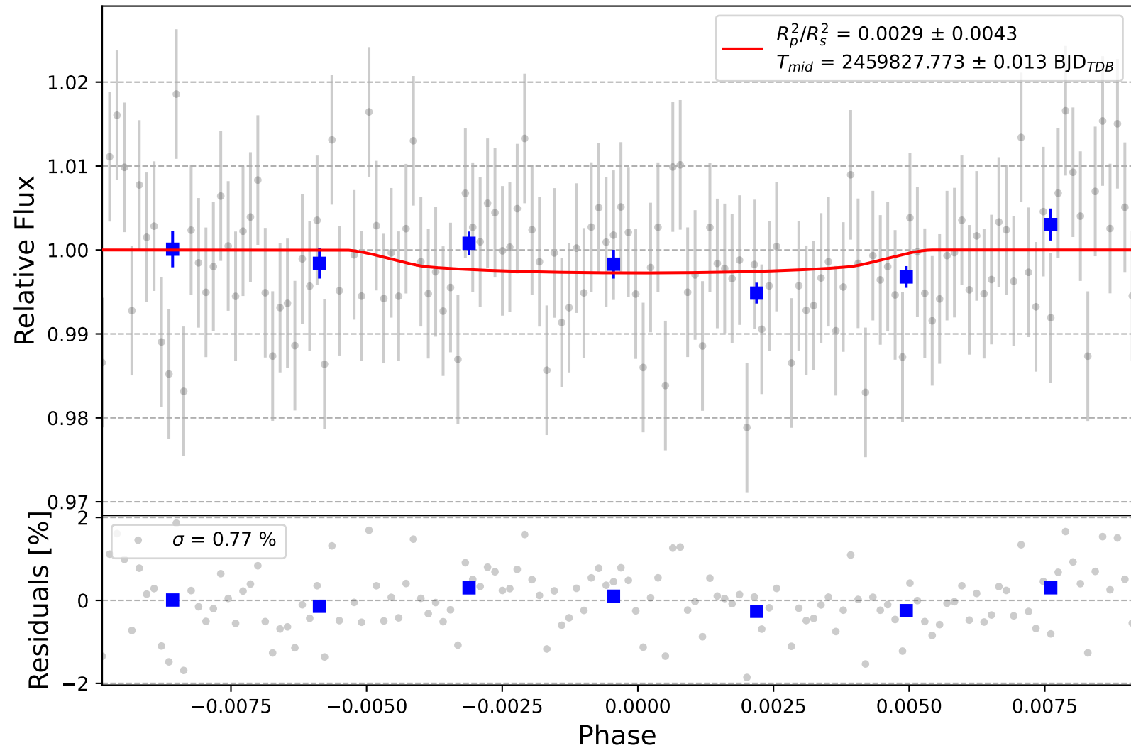
K2-141 c
