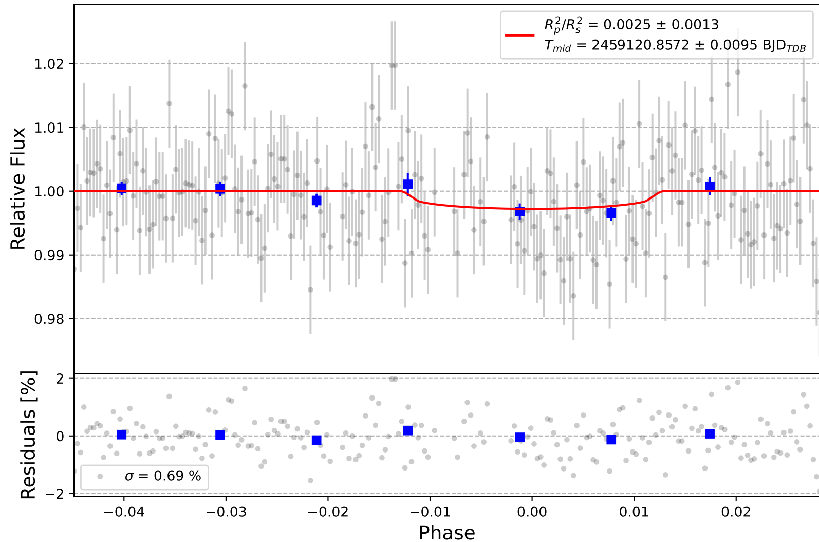
K2-216 b
