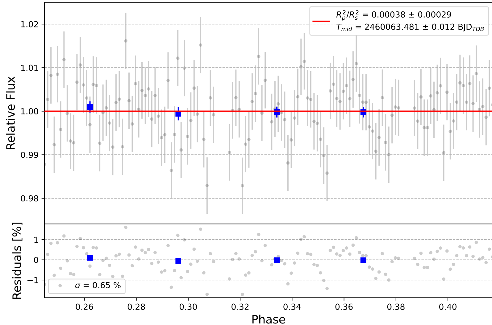
K2-229 b
