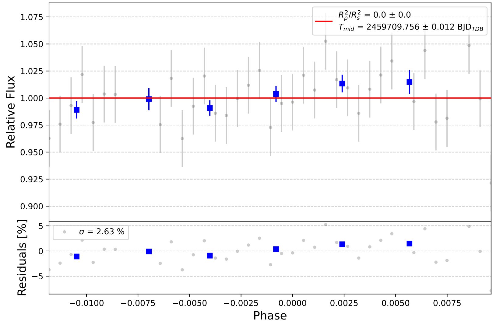
K2-242 b
