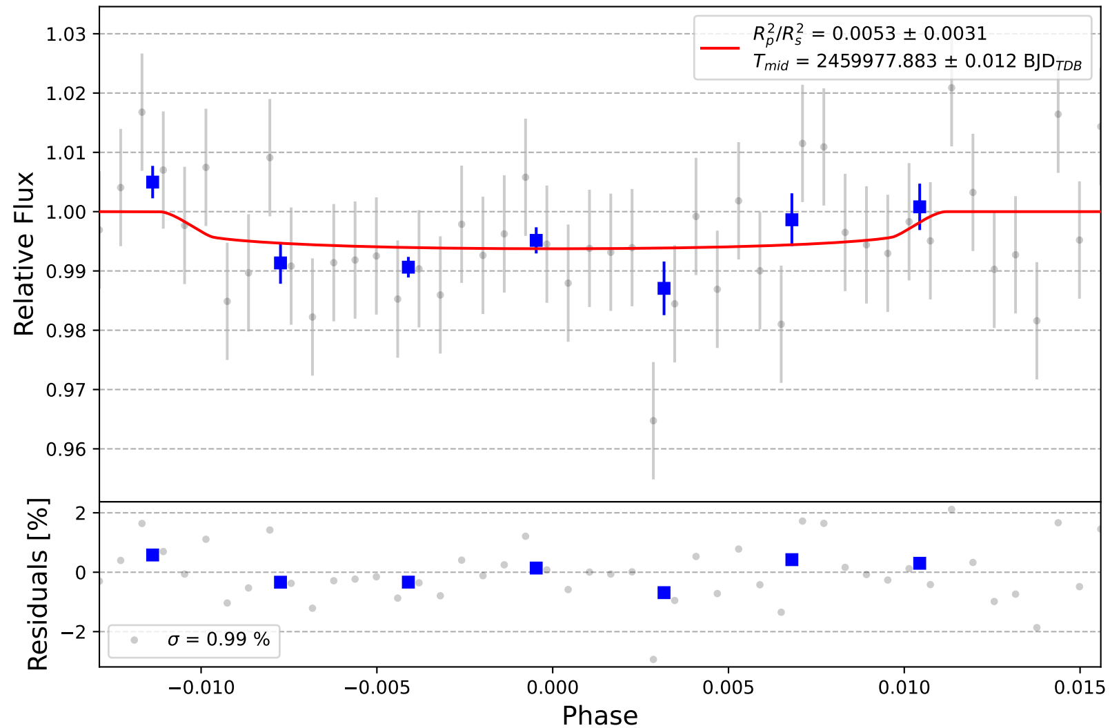
K2-246 b
