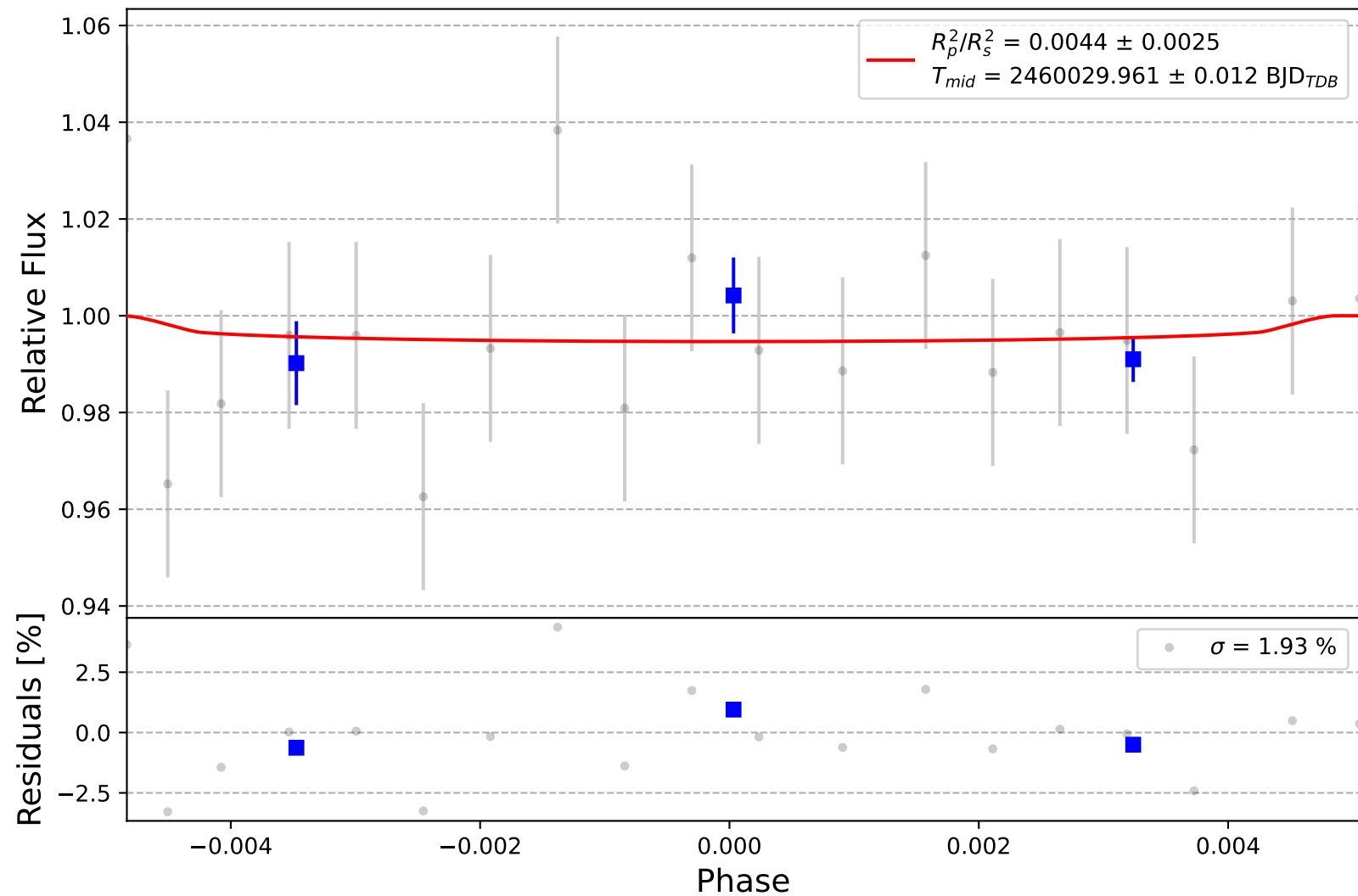
K2-247 c
