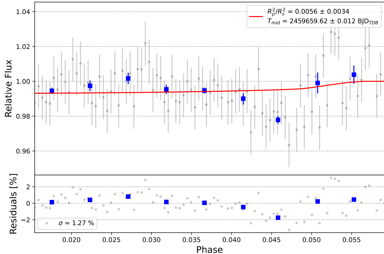
K2-270 c
