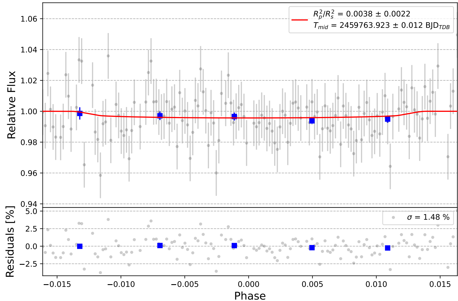
K2-285 b
