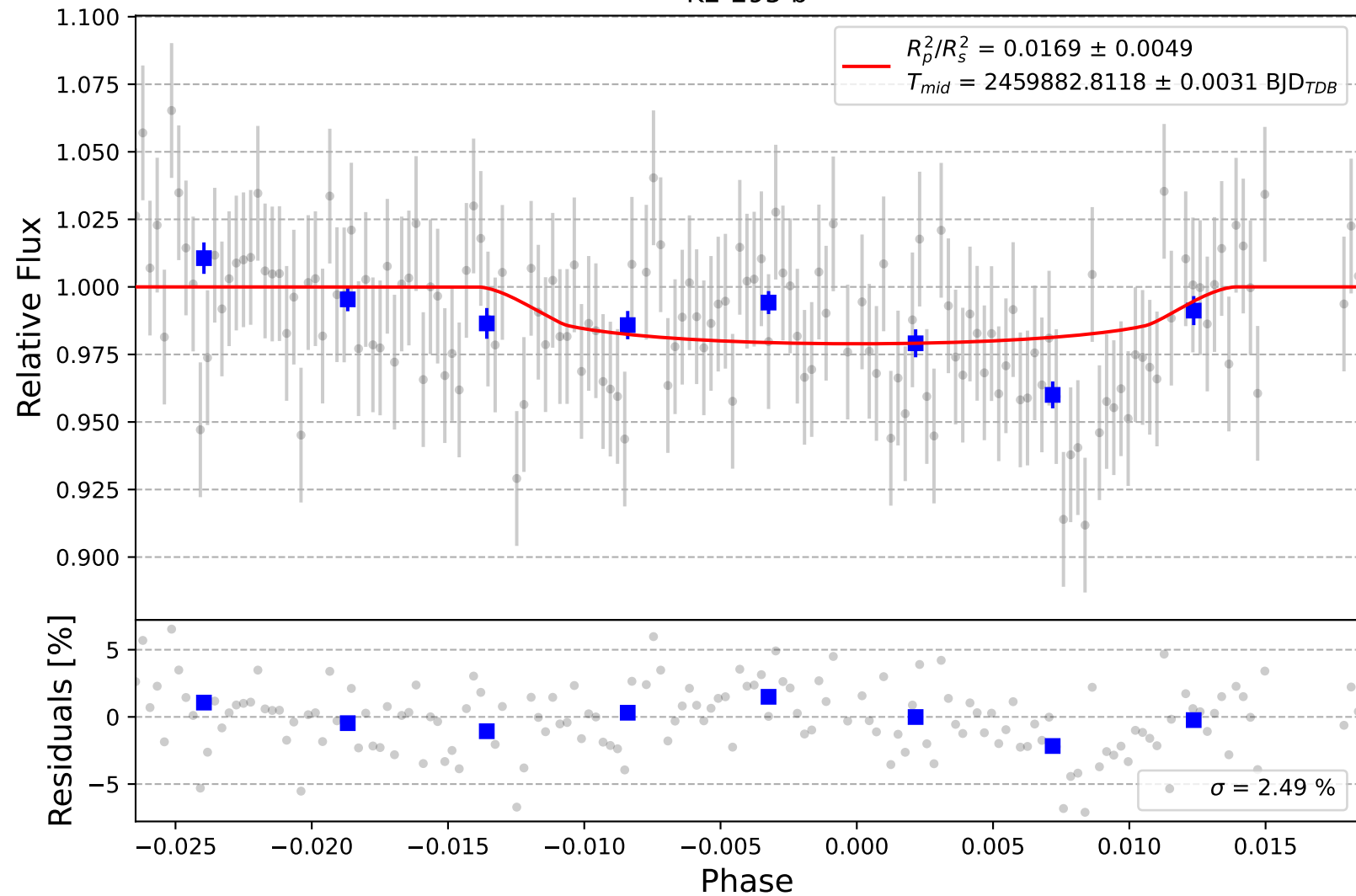
K2-295 b
