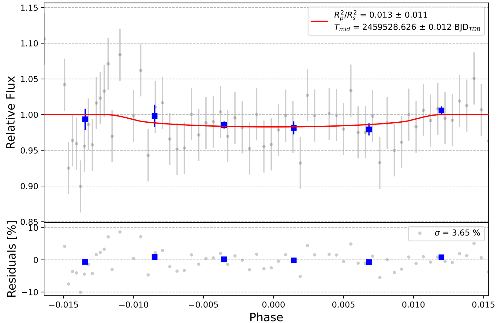
K2-295 b
