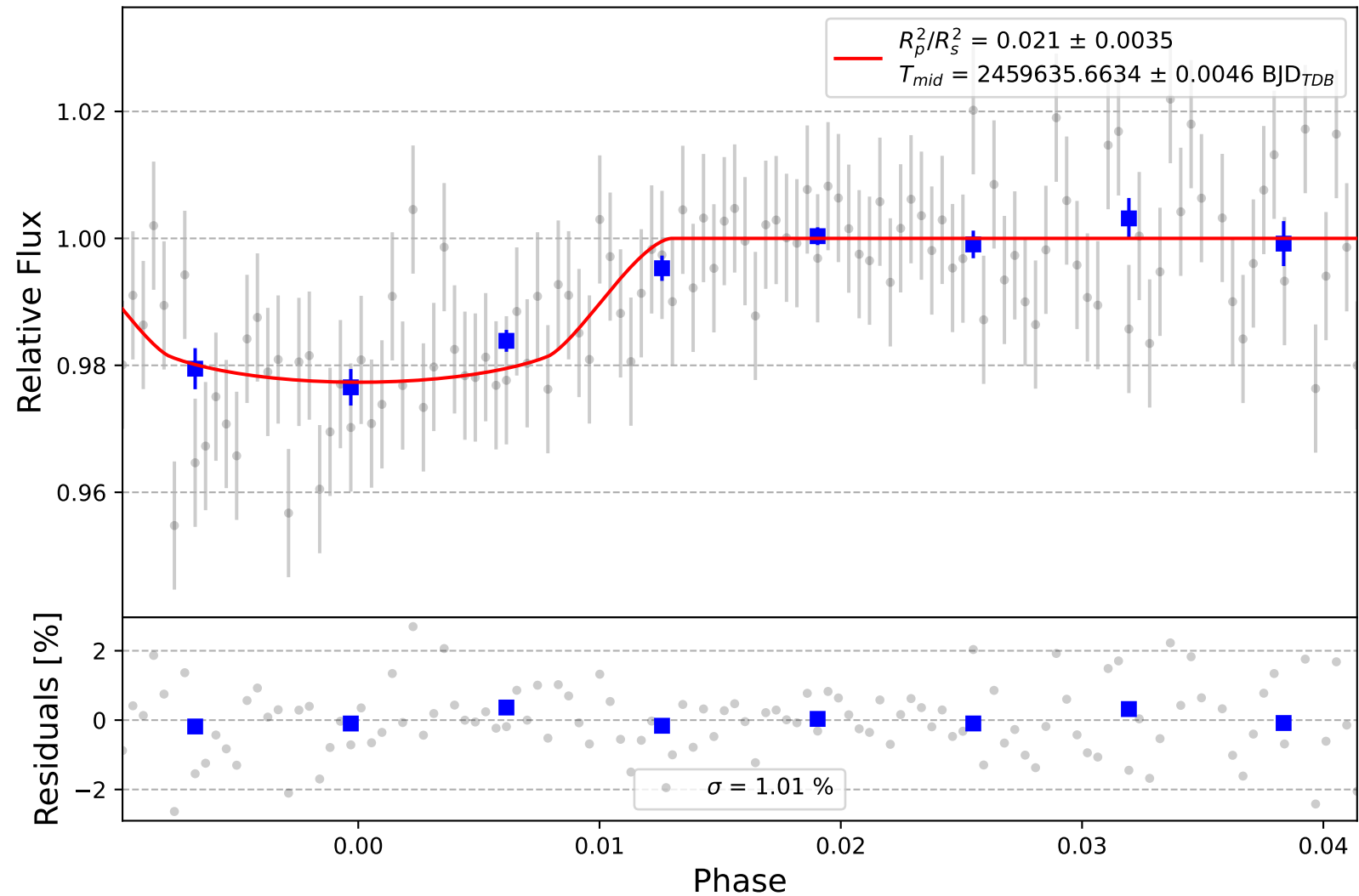
K2-29 b
