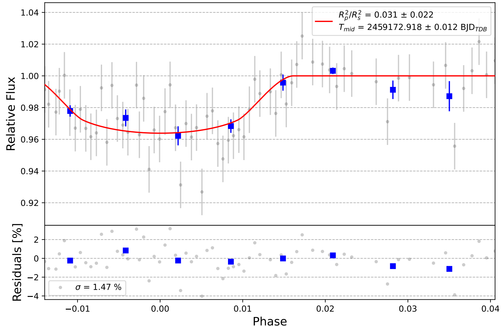
K2-29 b
